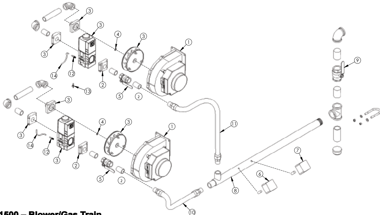
PFC-1500 – Blower/Gas Train
