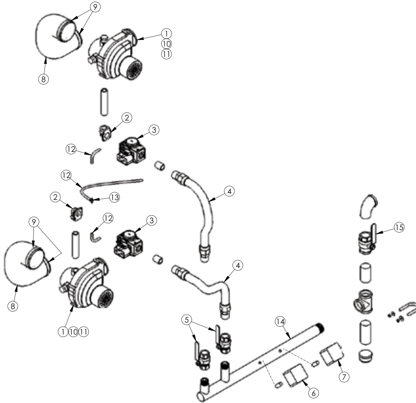
PFC-850/1000 – Blower/Gas Train
